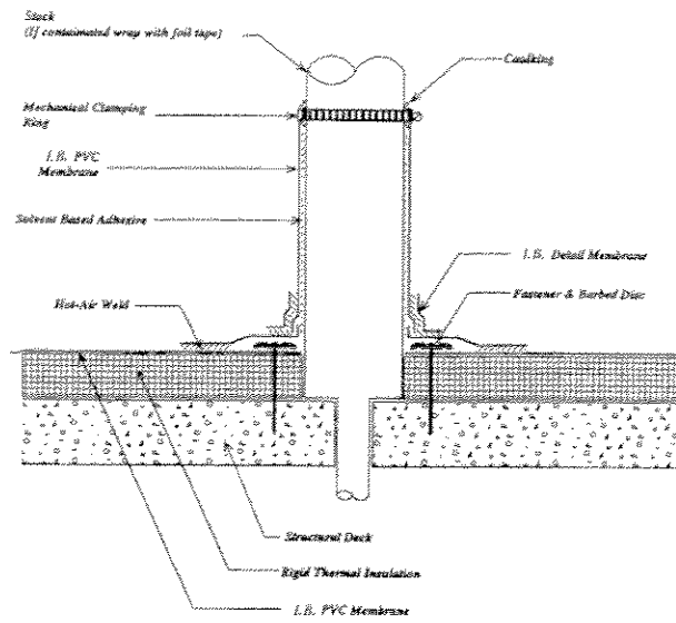
STACK FLASHING FABRICATED
