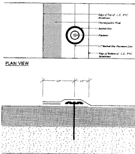
MECHANICALLY FASTENED INSEAM BARBED-DISC PLACEMENT
