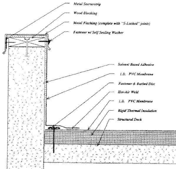
PARAPET WALL WITH METAL CAP
